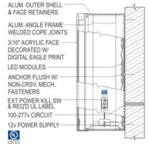
LED ILLUMINATED WALL SIGN
